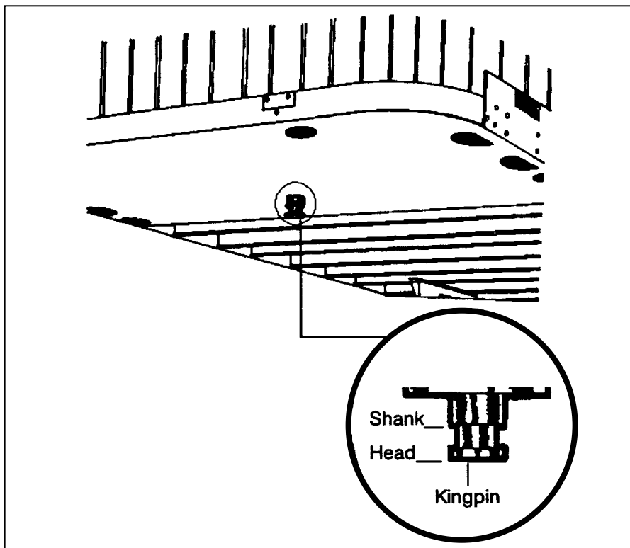
Figure 6-7 Trailer Kingpin
