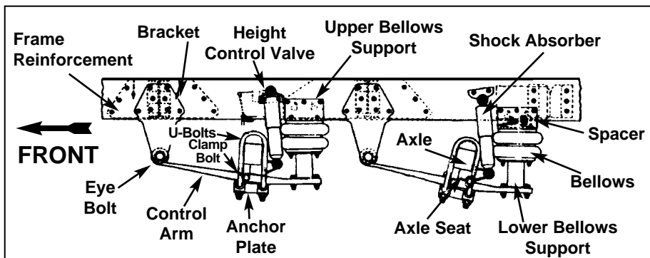
Figure 2-4 Air Suspension Parts
