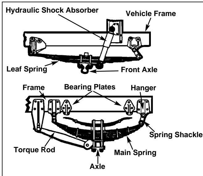
Figure 2-2 Key Suspension Parts
