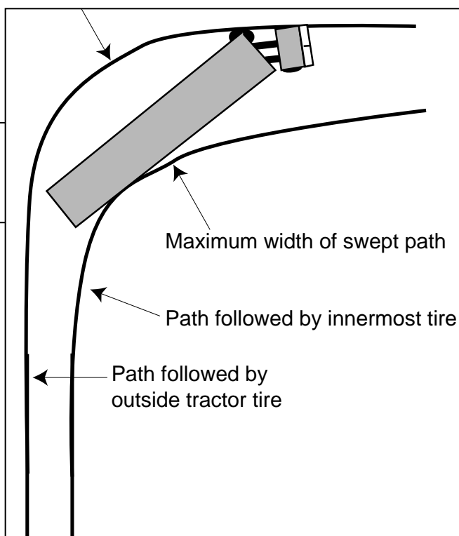
Figure 6-4 Offtracking in a 90-degree turn
