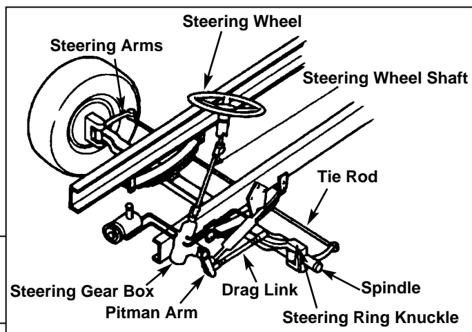
Figure 2-1 Examples of Steering System Key Parts
